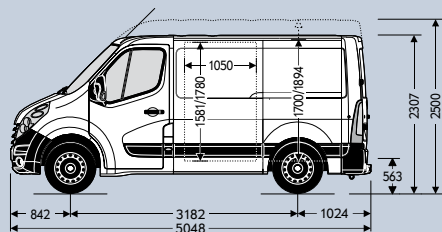
L1H1/H2 FWD
